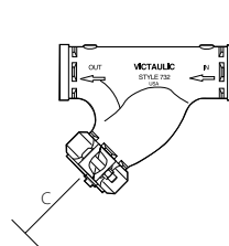
Series 732 Wye-Type Vic-Strainers Typical 2 – 12-inch/60.3 – 323.9-mm Sizes
