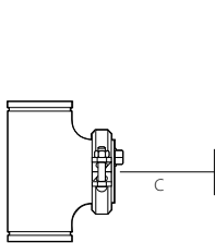
Series 730 Tee-Type Vic-Strainers Typical 1½ – 12-inch/48.3 – 323.9-mm Sizes
