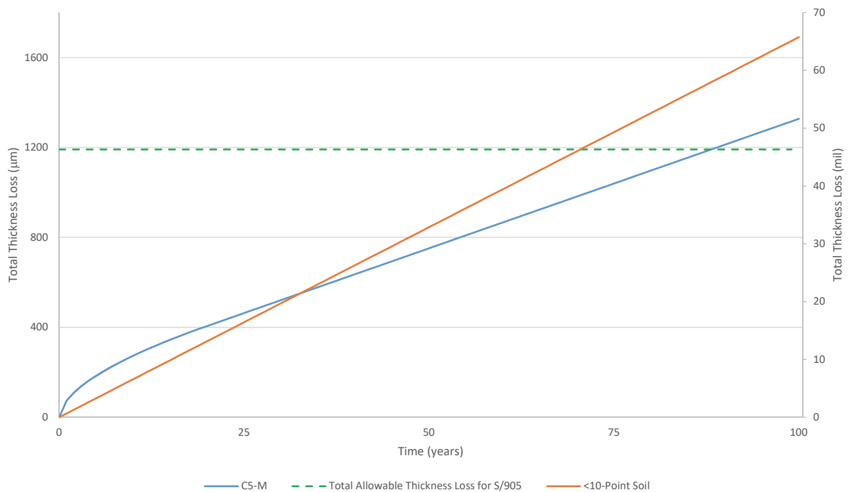
Figure 6: Useful Life Prediction for Victaulic fluoropolymer-coated bolt in C5-M and <10-point soil environments
