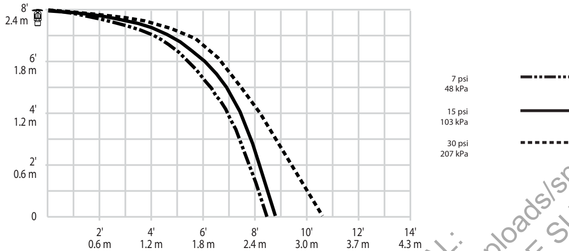
Models V3602, V3601 Upright Distribution Patterns – Trajectory
