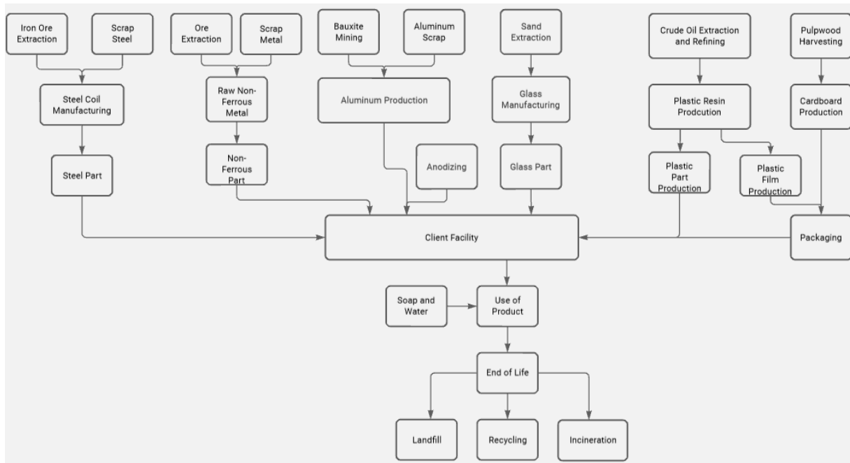
Figure 2. Visualization of material flows for Victaulic sprinkler head products.
